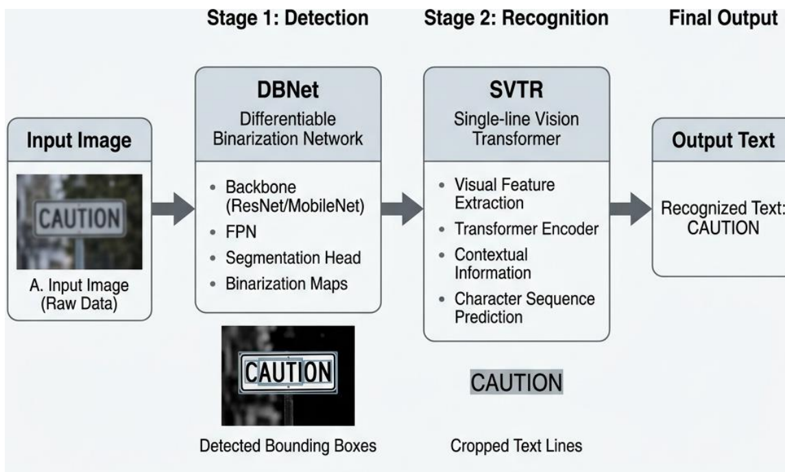
Figure 3: PaddleOCR Advanced Multi-Stage Architecture (DBNet + SVTR) (Source: Adapted from [4])
