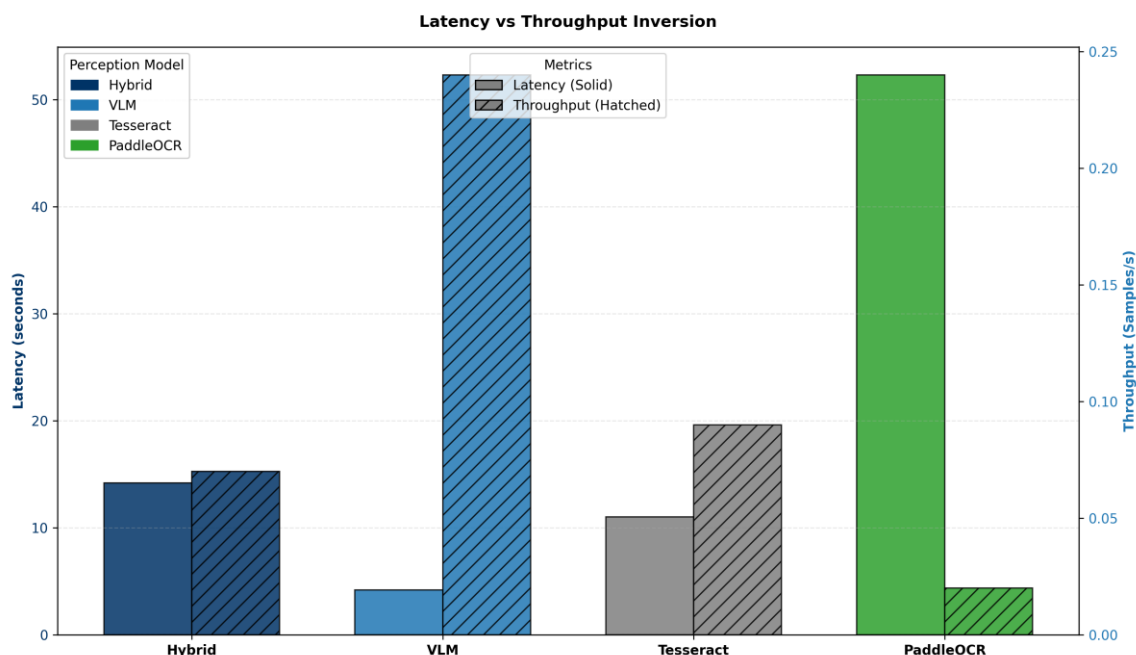
Figure 14: Latency vs Throughput Inversion (Source: Own elaboration)
