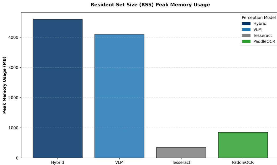
Figure 15: Resident Set Size (RSS) Peak Memory Usage (Source: Own elaboration)
